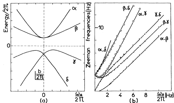
FIG. 17. ^{201}\text{Hg} atoms perturbed by a fictitious electric field perpendicular to the magnetic field. (a) Theoretical Zeeman diagram. (b) Variation of the Zeeman transition frequencies with \omega_0/2\pi . The theoretical curves are deduced from the diagram of Fig. 17(a). Crosses and open circles correspond to experimental points, determined, respectively, with a linear and circular polarization of B_2 .
