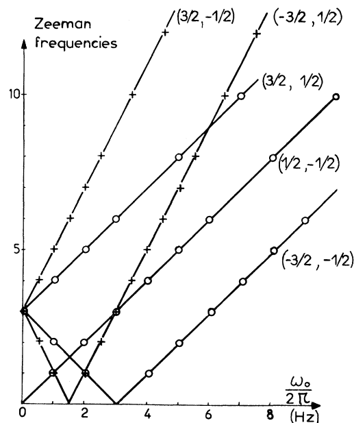
FIG. 16. Variation of the Zeeman transition frequencies with \omega_0/2\pi . Theoretical curves are deduced from the diagram of Fig. 14. Crosses and open circles correspond to experimental points, determined, respectively, with a linear and circular polarization of the pumping beam B_2 .
