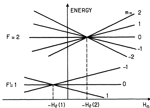
FIG. 9. Zeeman hyperfine diagram of ^{87}\text{Rb} atoms perturbed by B_1 ( \vec{H}_0 parallel to B_1 ). The two fictitious fields \vec{H}_f(1) and \vec{H}_f(2) , describing the effect of B_1 inside the F'=1 and F=2 hyperfine levels, are of opposite signs.
