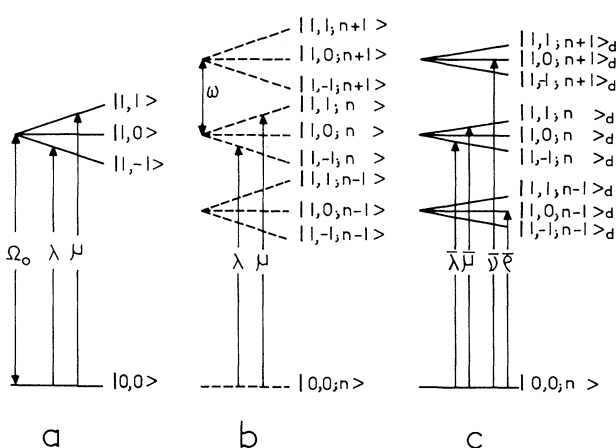
FIG. 2. (a) Hyperfine Zeeman diagram of the H ground state. (b) Energy levels |F, m_F; n\rangle of the "ground state + rf field" system, neglecting the coupling with the rf field. (c) Energy levels |F, m_F; n\rangle_d of the "dressed" hydrogen ground state. Note the change in the slope of the energy levels.
