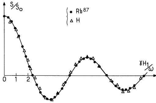
FIG. 3. Plot of the ratio s/s_0 as a function of \gamma H_1/\omega . The experimental points for \text{Rb}^{87} and \text{H} fit into the same theoretical curve.
