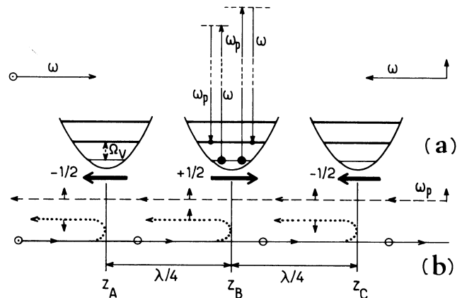
FIG. 2. (a) Bottom part of three adjacent optical potential wells for a F = \frac{1}{2} \rightarrow F' = \frac{3}{2} transition in a \text{lin} \perp \text{lin} pump configuration. These potential wells are alternatively associated with ground-state sublevels m_J = -\frac{1}{2} and m_J = \frac{1}{2} as shown in the figure. The magnetizations in successive planes have opposite signs as in an antiferromagnetic medium. The vertical arrows represent Raman processes between v=0 and v=1 vibrational levels, leading to an absorption or an amplification of the probe beam. More generally, all transitions v \rightarrow v \pm 1 contribute to the Raman lines shown in Figs. 1(b) and 1(c) in a way which depends on the probe polarization. This explains the difference in the widths of the Raman resonances. (b) Interpretation of the central narrow structure for the configuration of Fig. 1(c). The pump beam coming from the left (solid line) is backscattered by the magnetization planes in z_A , z_B , and z_C . The backscattered waves (dotted lines) undergo a rotation of polarization and can interfere with the probe wave coming from the right (dashed line). The change of sign of the magnetization (represented by a bold arrow) compensates for the \pi phase shift due to propagation between successive planes.
