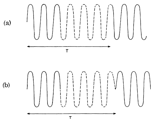
FIG. 1. (a) Two Fourier-limited time-delayed pulses generated by amplifying the same cw wave by two time-delayed independent pulsed amplifiers. They clearly have the same phase which is that of the cw carrier. (b) Two pulses originated from the same Fourier-limited pulse by using a delay line. The second one is just the time translation of the first one by an amount T . The phase difference between the two pulses clearly depends on \omega T .
