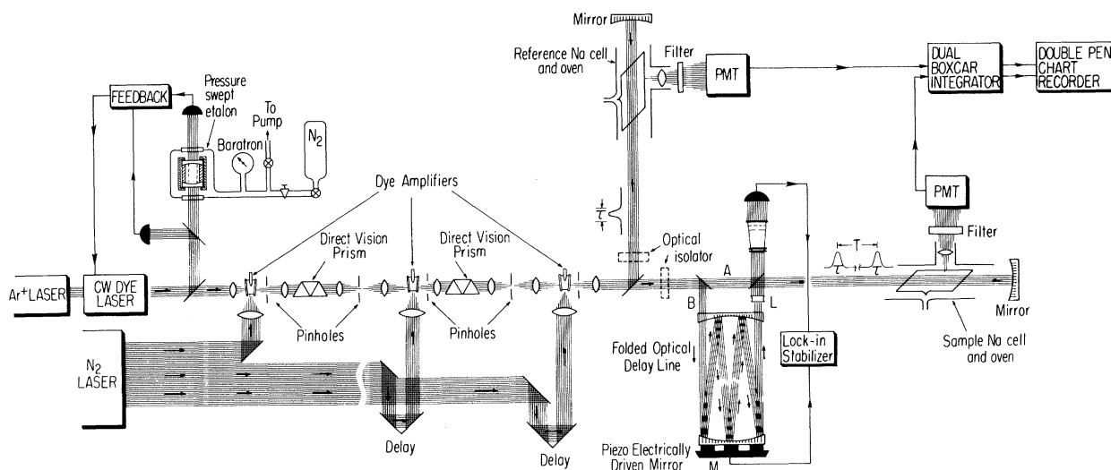
FIG. 2. The experimental setup.
