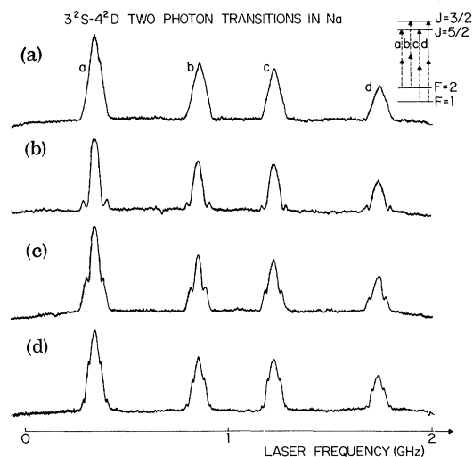
FIG. 3. (a) Recording of the four Doppler-free 3^2S - 4^2D two-photon resonances of Na observed in the reference cell excited with a single pulse. (b)–(d) Same resonances observed in the sample cell excited with two time-delayed coherent pulses. Width of each pulse, \tau = 8 nsec; effective delay between two pulses, \tau_{\text{eff}} = 2T = 17, 25 , and 33 nsec, respectively. The spacing between the fringes, \Delta\nu \approx 60, 40 , and 30 MHz, respectively, is in good agreement with the theoretical prediction 1/2T .
