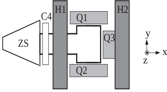
Fig. 2. Magnetostatic trap. ZS is the Zeeman slower coil, Q1, Q2 and Q3 the Ioffé-Prichard coils, H1 and H2 are the bias compensation coils. C4 is a coil used to compensate the field created by ZS at the center of the cell.
