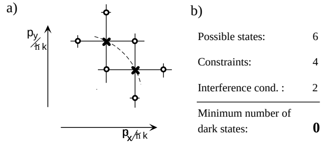
Fig. 5. Disposition of isolated pairs in the plane (p_x/\hbar k) - (p_y/\hbar k) in momentum space that appear when looking for intersections between the circles of radii larger than \sqrt{5} .
