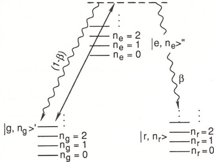
Fig. 3. Diagram for the cooling when the motion is quantized. Each electronic state has a sublevel structure of harmonic-oscillator levels labeled by the quantum numbers n_j , where j = g, e , or r . Cooling is represented by scattering processes of the form n_g \rightarrow n_e \rightarrow n_r , where n_r < n_g . This may be viewed as due to spontaneous Raman scattering off states |g, n_g\rangle' and |e, n_e\rangle'' , which are dressed by the laser.
