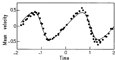
FIG. 13. Bloch oscillations of atoms in a periodic optical potential (from Ben Dahan et al. , 1996). Mean velocity (in units of the recoil velocity) vs time (in units of half the Bloch period) for ultracold cesium atoms moving in a periodic optical potential and submitted in addition to a constant force.
