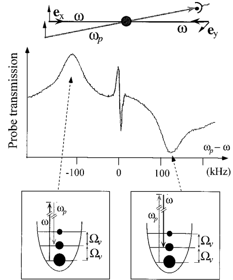
FIG. 4. Probe absorption spectrum of a 1D optical lattice (from Verkerk et al. , 1992). The upper part of the figure shows the two counterpropagating laser beams with frequency \omega and orthogonal linear polarizations forming the 1D optical lattice, and the probe beam with frequency \omega_p whose absorption is measured by a detector. The lower part of the figure shows the probe transmission vs \omega_p - \omega . The two lateral resonances corresponding to amplification or absorption of the probe are due to stimulated Raman processes between vibrational levels of the atoms trapped in the light field (see the two insets). The central narrow structure is a Rayleigh line due to the antiferromagnetic spatial order of the atoms.
