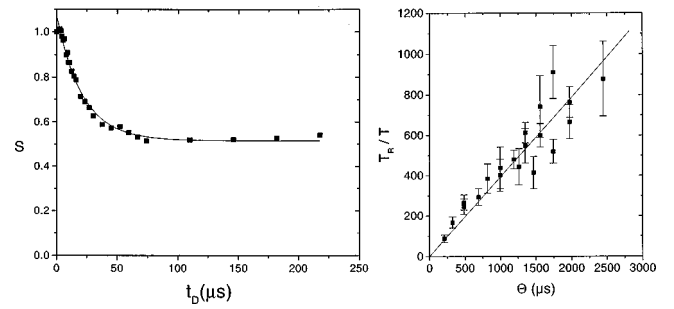
FIG. 8. Measurement of the spatial correlation function of atoms cooled by VSCPT (from Saubamea et al. , 1997). After a cooling period of duration \theta , the two VSCPT beams are switched off during a dark period of duration t_D . The two coherent wave packets into which atoms are pumped fly apart with a relative velocity 2v_R and get separated by a distance a = 2v_R t_D . Reapplying the two VSCPT beams during a short probe pulse, one measures a signal S which can be shown to be equal to [1 + G(a)]/2 where G(a) is the spatial overlap between the two identical wave packets separated by a . From G(a) , which is the spatial correlation function of each wave packet, one determines the atomic momentum distribution which is the Fourier transform of G(a) . The left part of the figure gives S vs a . The right part of the figure gives T_R/T vs the cooling time \theta , where T_R is the recoil temperature and T the temperature of the cooled atoms determined from the width of G(a) . The straight line is a linear fit in agreement with the theoretical predictions of Lévy statistics. The lowest temperature, on the order of T_R/800 , is equal to 5 nK.
