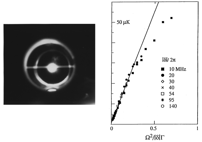
FIG. 3. Temperature measurements in cesium optical molasses (from Salomon et al. , 1990). The left part of the figure shows the fluorescence light emitted by the molasses observed through a window of the vacuum chamber. The horizontal bright line is the fluorescence light emitted by the atomic beam which feeds the molasses and which is slowed down by a frequency chirped laser beam. Right part of the figure: temperature of the atoms measured by a time-of-flight technique vs the dimensionless parameter \Omega^2/|\delta|\Gamma proportional to the light shift ( \Omega is the optical Rabi frequency, \delta the detuning and \Gamma the natural width of the excited state).
