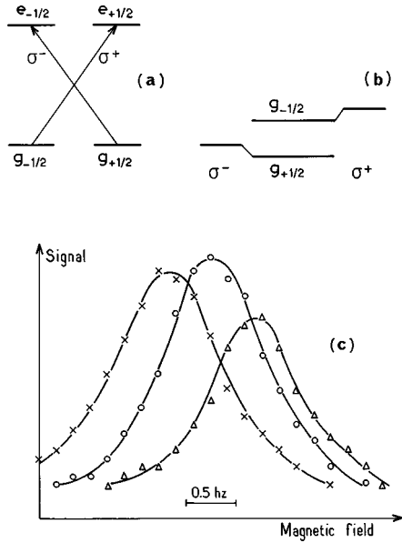
FIG. 1. Experimental observation of light shifts (from Cohen-Tannoudji, 1961). For a J_g = 1/2 \leftrightarrow J_e = 1/2 transition (a), a \sigma^+ -polarized nonresonant excitation shifts only the sublevel g_{-1/2} [right part of (b)] whereas a \sigma^- -polarized excitation shifts only the sublevel g_{+1/2} [left part of (b)]. The detuning \delta is positive and very large compared to the Zeeman splittings in e and g . The Zeeman splitting in the ground state is thus increased in the first case, decreased in the second one. (c) magnetic resonance signal vs magnetic field, in units of the corresponding Larmor frequency. The central curve (circles) is the resonance curve in the absence of light shift. When the nonresonant light beam is introduced, either \sigma^+ -polarized (crosses) or \sigma^- -polarized (triangles), the magnetic resonance curve is light shifted in opposite directions.
