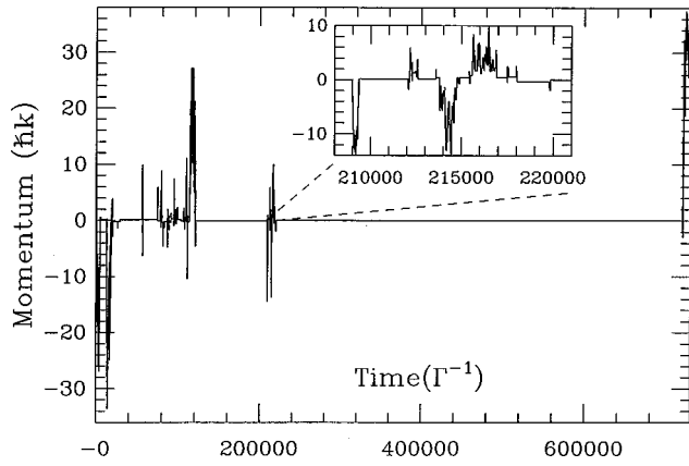
FIG. 10. Monte Carlo wave function simulation of one-dimensional VSCPT (from Bardou, Bouchaud et al. , 1994). Momentum p characterizing the cooled atoms vs time. Each vertical discontinuity corresponds to a spontaneous emission jump during which p changes in a random way. Between two successive jumps, p remains constant. The inset shows a zoomed part of the sequence.
