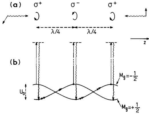
FIG. 2. Sisyphus cooling. Laser configuration formed by two counterpropagating plane waves along the z axis with orthogonal linear polarizations (a). The polarization of the resulting electric field is spatially modulated with a period \lambda/2 . Every \lambda/4 , it changes from \sigma^+ to \sigma^- and vice versa. For an atom with two ground state Zeeman sublevels M_g = \pm 1/2 , the spatial modulation of the laser polarization results in correlated spatial modulations of the light shifts of these two sublevels and of the optical pumping rates between them (b). Because of these correlations, a moving atom runs up potential hills more frequently than down [double arrows of (b)].
