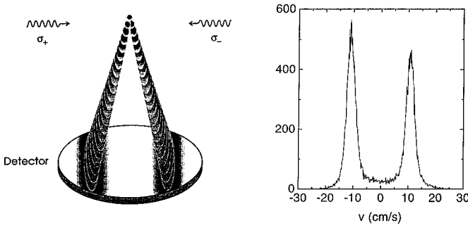
FIG. 7. One-dimensional Velocity Selective Coherent Population Trapping (VSCPT) experiment. The left part of the figure shows the experimental scheme. The cloud of precooled trapped atoms is released while the two counterpropagating VSCPT beams with orthogonal circular polarizations are applied during a time \theta=1 ms. The atoms then fall freely and their positions are detected 6.5 cm below on a microchannel plate. The double band pattern is a signature of the 1D cooling process which accumulates the atoms in a state which is a linear superposition of two different momenta. The right part of the figure gives the velocity distribution of the atoms detected by the microchannel plate. The width \delta v of the two peaks is clearly smaller than their separation 2v_R , where v_R=9.2 cm/s is the recoil velocity. This is a clear signature of subrecoil cooling.
