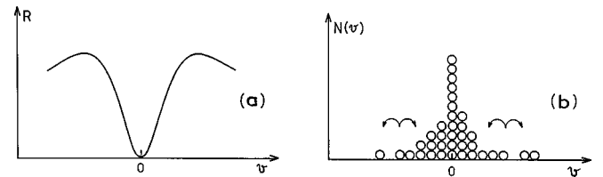
FIG. 5. Subrecoil laser cooling. (a) the random walk of the atom in velocity space is supposed to be characterized by a jump rate R which vanishes for v=0 . (b) as a result of this inhomogeneous random walk, atoms which fall in a small interval around v=0 remain trapped there for a long time, on the order of [R(v)]^{-1} , and accumulate.
