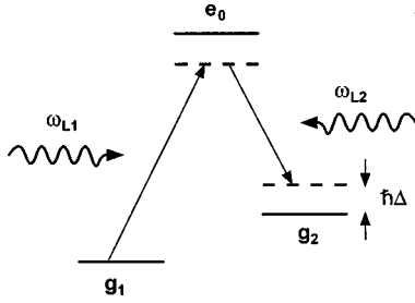
FIG. 6. Coherent population trapping. A three-level atom g_1, g_2, e_0 is driven by two laser fields with frequencies \omega_{L1} and \omega_{L2} exciting the transitions g_1 \leftrightarrow e_0 and g_2 \leftrightarrow e_0 , respectively. \hbar\Delta is the detuning from resonance for the stimulated Raman process induced between g_1 and g_2 by the two laser fields \omega_{L1} and \omega_{L2} . When \Delta=0 , atoms are optically pumped in a linear superposition of g_1 and g_2 which no longer absorbs light because of a destructive interference between the two absorption amplitudes g_1 \rightarrow e_0 and g_2 \rightarrow e_0 .
