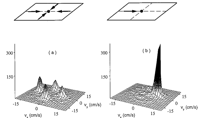
FIG. 9. Two-dimensional VSCPT experiment (from Kulin et al. , 1997). The experimental scheme is the same as in Fig. 7, but one uses now four VSCPT beams in a horizontal plane and atoms are pumped into a linear superposition of four different momentum states, giving rise to four peaks in the two-dimensional velocity distribution (a). When three of the four VSCPT laser beams are adiabatically switched off, the whole atomic population is transferred into a single wave packet (b).
