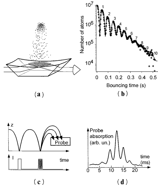
FIG. 12. Gravitational cavity for neutral atoms (from Aminoff et al. , 1993, and Steane et al. , 1995). (a) trampoline for atoms. Atoms released from a magneto-optical trap bounce off a concave mirror formed by a blue detuned evanescent wave at the surface of a curved glass prism. (b) number of atoms at the initial position of the trap vs time after the trap has been switched off. Ten successive bounces are visible in the figure. (c) principle of the experiment demonstrating the frequency modulation of de Broglie waves. The upper trace gives the atomic trajectories (vertical position z vs time). The lower trace gives the time dependence of the intensity I of the evanescent wave. The first pulse is used for making a velocity selection. The second pulse is modulated in intensity. This produces a vibrating mirror, giving rise to a frequency-modulated reflected de Broglie wave which consists in a carrier and sidebands at the modulation frequency. The energy spectrum of the reflected particles is thus discrete so that the trajectories of the reflected particles form a discrete set. (d) this effect is detected by looking at the time dependence of the absorption of a probe beam located above the prism.
