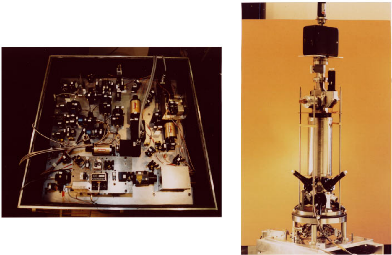
FIG. 11. (Color) The microgravity clock prototype. The left part is the 60 cm×60 cm×15 cm optical bench containing the diode laser sources and the various optical components. The right part is the clock itself (about one meter long) containing the optical molasses, the microwave cavity and the detection region.
