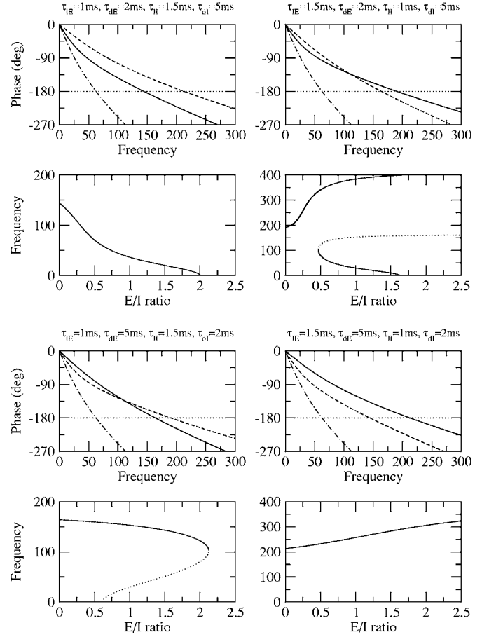
FIG. 8. Effect of excitation/inhibition balance on network frequency, for four different sets of synaptic time constants, indicated on top of the phase vs frequency panels (rise times are 0.5 ms in all panels). For each set, we show the synaptic phase shift of inhibitory (solid) and excitatory (dashed) synapses, together with the sum of the two (dot-dashed). The intersection of the solid curve with the horizontal dotted line indicates the frequency of a purely inhibitory network, while the intersection of the dot-dashed curve and the dotted line indicate the frequency of a network with E-I loop only. We also show how the network frequency depends on the E/I ratio \alpha . Note the different qualitative behaviors as a function of relative time constants. Top left: excitation is faster than inhibition: frequency decreases with E/I ratio. Top right: inhibition has shorter latency but longer decay time: frequency first increases, then jumps discontinuously to a much lower ( <100 Hz) frequency, and then decreases. Bottom left: inhibition has longer latency but shorter decay time, frequency decreases with E/I ratio. Bottom right: inhibition is faster than excitation: frequency increases with E/I ratio.
