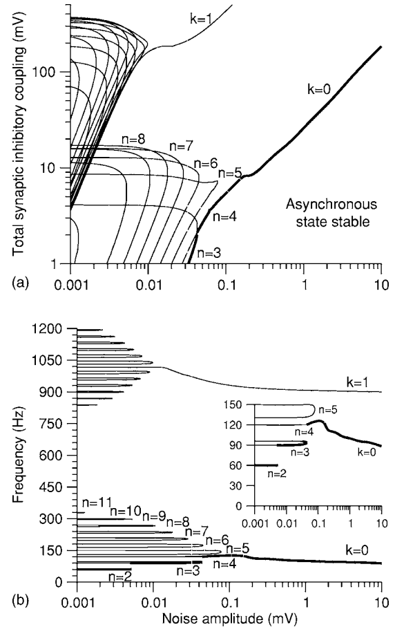
FIG. 5. (a) Lines on which eigenmodes become unstable, obtained from Eq. (11), in the plane J - \sigma , for the parameters of Fig. 4. The asynchronous state is stable below the lowest line (region marked “asynchronous state stable”). Several solutions of families to Eq. (11) exist, and are indexed by an integer k such that \Phi_S(\omega) + \Phi_R(\omega) + (2k+1)\pi = 0 . Only lines corresponding to families of solutions at k=0 and k=1 (marked in the figure) are indicated. Each family is composed of individual branches labeled by integer values of n (indicated only for k=0 ). (b) Frequency of marginal modes. The thick curve in (a) is the stability boundary of the asynchronous state. The thick curve in (b) is the frequency of the unstable mode on this boundary plotted against the noise. Adapted from Ref. 11.
