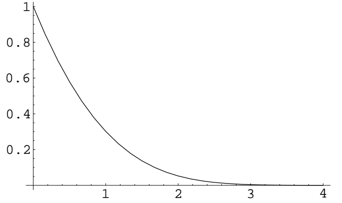
FIG. 13: The fixed-point function y_1(u) at 1-loop order for non-periodic disorder.
