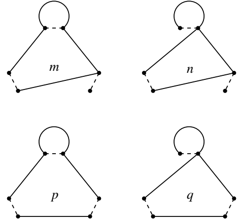
FIG. 9: 2-loop diagrams of class C
