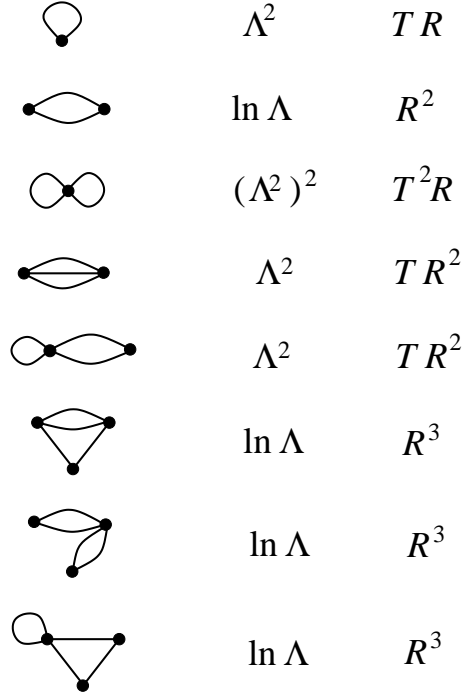
FIG. 19: Divergent unsplitted diagrams to one and two loops.
