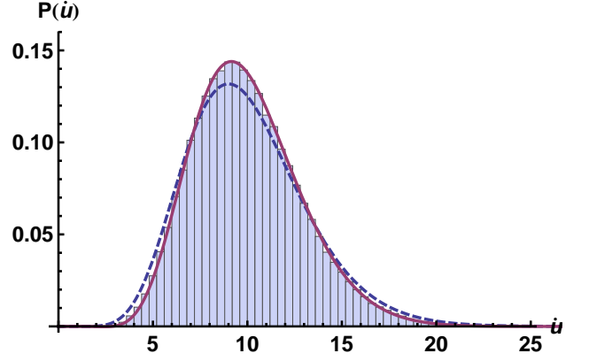
FIG. 3: Single-particle velocity distribution P(\dot{u}) in the 2-particle toy model for weak elasticity. Histogram: Numerical results from simulations for k = 0.2 . Dashed line: Stationary distribution in absence of elastic coupling ( k = 0 ). Solid (red) line: \mathcal{O}(k) result from (62).
