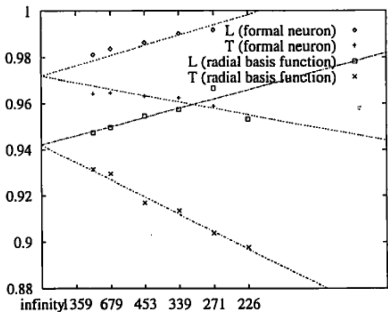
Fig. 4. Success rate (after pruning) versus inverse of data size S for three choices of classifiers.
