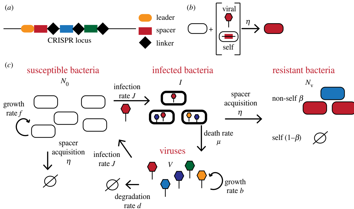
Figure 1. Cartoon representation of the CRISPR-Cas system model. (a) Bacteria protect themselves from surrounding phage viruses, V , by uptaking segments of their DNA and incorporating them into their genome. The uptaken spacers (coloured rectangles) are incorporated into the CRISPR locus and separated by linkers (black diamonds). (b) A susceptible bacterium (empty oval) can take up viral DNA spacers from the red phage (top) or its own DNA as spacers from its own genome (bottom). The acquisition rate of any new spacer is \eta . Note that we define our rates as the proportionality constant to the number of individuals in the reacting populations, as is customary in chemical kinetics. Our rates have units of inverse time. (c) In a given viral environment, a number N of bacteria do not carry protection and are phage susceptible (empty ovals), they can get infected (empty ovals with viruses) and after acquisition bacteria become resistant with the appropriate anti-phage spacers (coloured ovals). All bacteria reproduce at a maximum growth rate f up to carrying capacity K . Susceptible bacteria become infected with rate J or they acquire a self-targeting spacer with rate \eta (since they are not infected they can only acquire self-targeting spacers). Infected cells can acquire a spacer with rate \eta and become resistant with probability \beta or die due to autoimmunity from self-spacers. Infected cells that do not acquire spacers die at a rate \mu producing B new virus copies. We assume there are two types of spacers: the self-targeting spacers of bacterial origin, which lead to the death of the bacteria through auto-immunity, and a proportion of phage-targeting spacers uptaken with probability \beta , whose incorporation turns susceptible bacteria into protected ones. (Online version in colour.)
