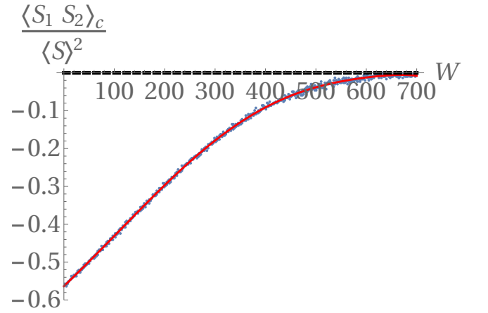
FIG. 7: Comparison between the measurement of the normalized moment \frac{\langle S_1 S_2 \rangle_{\rho_W^c}}{\langle S \rangle_{\rho}^2} (blue dots) and the prediction from the exact result (39) using the measurement of \Delta(u) (red curve) in the RF toy model. The agreement is perfect as expected.
