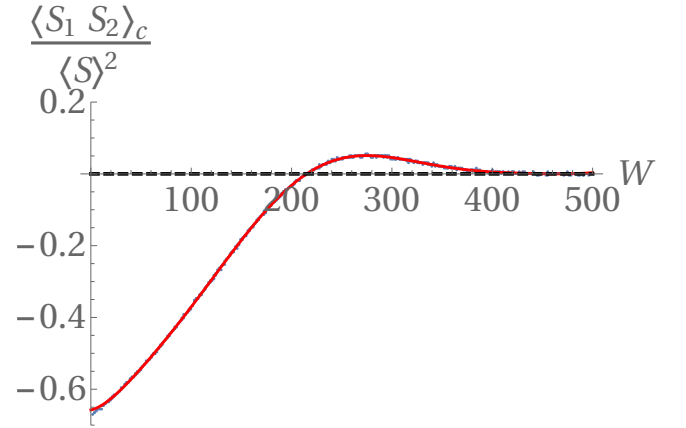
FIG. 3: Comparison between the measurement of the normalized moment \frac{\langle S_1 S_2 \rangle_{\rho_W^c}}{\langle S \rangle_{\rho}^2} (blue dots) and the prediction from the exact result (39) using the measurement of \Delta(u) (red curve) in the RB toy model. The agreement is perfect as expected.
