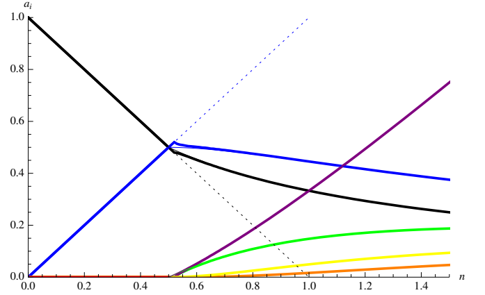
FIG. 14: The phase diagram for r = 6 . The transition is at n_c = 0.517 . Figure to be compared to Fig. 8. The thin underlying lines are the MF solution, the thin dotted lines the unstable solution.
