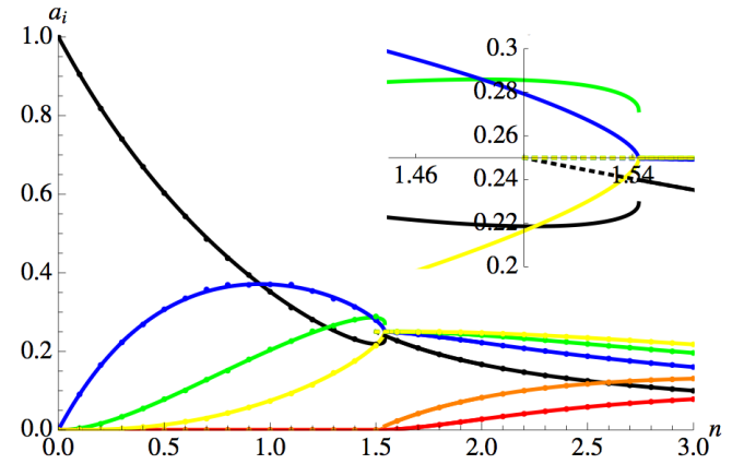
FIG. 12: Main plot: The phase diagram for the MF version of the 2d-ASM. The branch starting at n = 1.5 , and a_{i,i \leq 3} = \frac{1}{4} is the MF solution (D5) ff. The branch starting at n = 0 was obtained by a direct numerical integration of the rate eqs. (D3), setting to zero all a_{i,i > 100} , and waiting until a steady state is reached. The dots are the result of a direct MC simulation of the MF-ASM model, starting from a Poisson distribution; we randomly distributed n times \text{size}^2 grains on a lattice of size 150. Note that Eqs. (D3) allow to predict the state reached by Monte Carlo. Also note that the branch with a_{i,i \geq 4} = 0 , which exists up to n \leq 3 , remains attractive beyond n = \frac{3}{2} (see inset, solid lines). The dashed lines are the solution (D5) ff.
