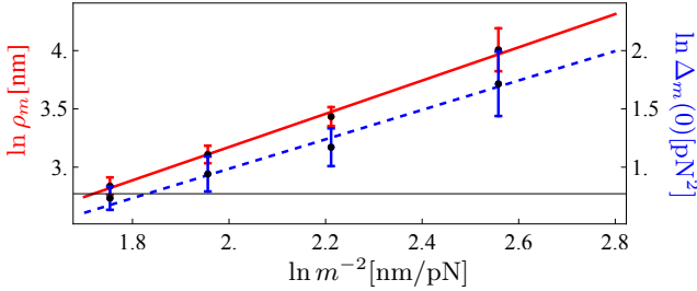
FIG. 5. Top: Properties of the force correlator for the four regions in Fig. 2. The correlation length \rho_m = C\Delta_m(0)/\Delta'_m(0) , with C = \tilde{\Delta}_m(0)/\tilde{\Delta}'_m(0) = 1.36 , see Eq. (7). Bottom: The scaling with m of \rho_m (red, solid), \zeta = 1.41 \pm 0.10 , and \Delta_m(0) (blue dashed), \zeta = 1.29 \pm 0.08 . Their mean \zeta = 1.34 \pm 0.06 agrees with the expected value, \zeta = 4/3 .
