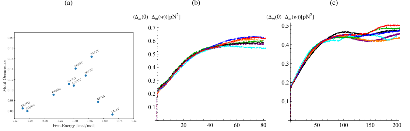
FIG. 7. (a) Distribution of the nearest-neighbour binding energies at 1M NaCl salt concentration for the 6 kbp sequence studied here. For the first (b) and third (c) region, the averaged \Delta_m for each salt concentration. Despite the dependence of the pinning force on the salt concentration, the correlation length is not visibly affected by the salt concentration. Color code as in Fig. 1 (c).
