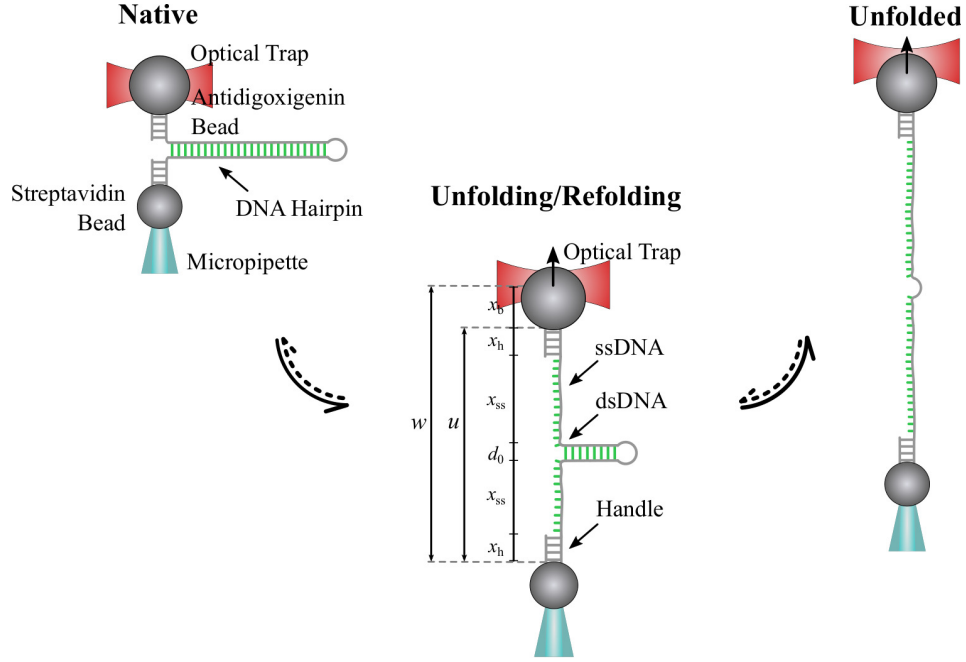
FIG. 6. Schematic description of the unzipping experiment as reported Appendix A and representation of the parameters introduced in the computation in Appendix B. As reported in the text, x_h is the extension of the handles, x_b is the displacement of the bead from the center of the optical trap, d_0 is the diameter of the folded double-helix ( \sim 2\text{nm} ) and x_{ss} is the extension of the ssDNA.
