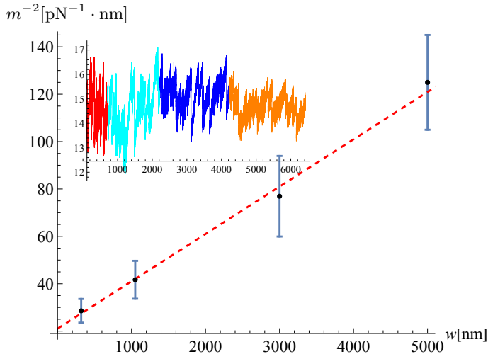
FIG. 2. Variation of the effective stiffness m^2 versus w according to Eq. (3). The points correspond to the measured values of 1/m^2 for the four FDC regions (each one shown with a different colour in the inset). The fit to data (dashed line) and the extrapolation to w = 0 gives the stiffness of the optical trap, k_b = 0.05 \pm 0.01\text{pN} \cdot \text{nm}^{-1} . The inset illustrates the four studied regions in a FDC at 1M NaCl.
