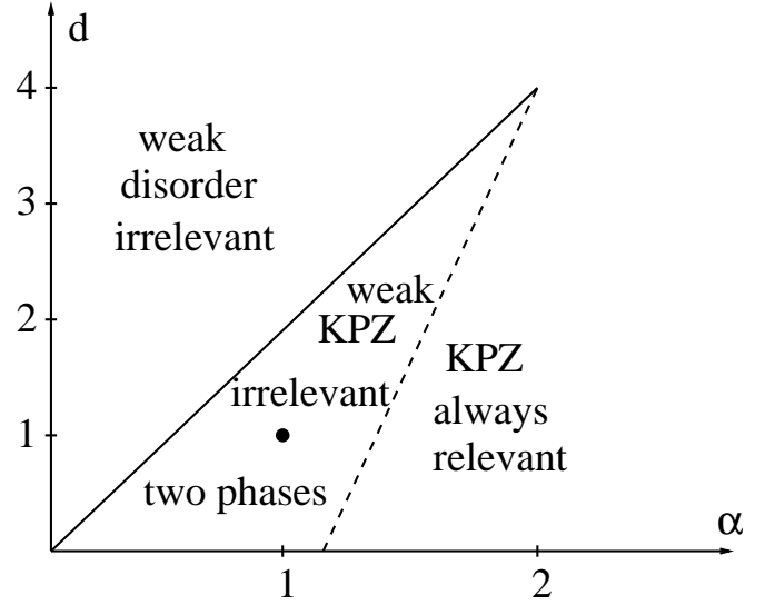
FIG. 12: Phase-diagram in the (\alpha, d) -plane. The solid line is \epsilon = 0 . The dashed line corresponding to (139) separates the domain where an infinitesimal KPZ-term is relevant from those where it is irrelevant. At order \epsilon^2 this line will bend to the left, but should not cross the point d = 1 and \alpha = 1 .
