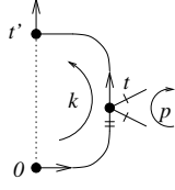
FIG. 1: The diagram generating the irreversible nonlinear KPZ term with one disorder vertex (notations are as in Ref. [18, 19]) and one c_4 vertex (the bars denote spatial derivatives).
