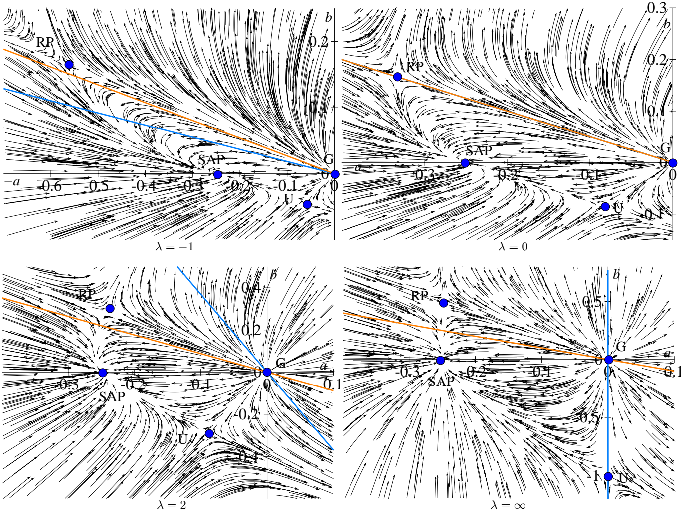
FIG. 6: Fixed point structure for different values of \lambda . The coordinate system is such that a grows to the right and b to the top. The both separatrices are b = -\frac{1}{2}ae^\lambda (blue/dark) and b = -a/(1 + e^{-\lambda}) (orange/bright).
