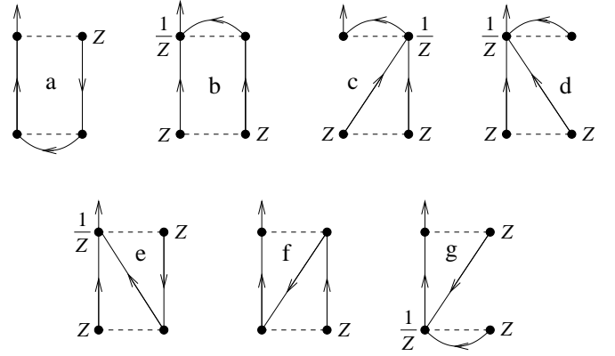
FIG. 4: 2-loop dynamical diagrams correcting the single \hat{Z} -component. Diagrams a – g correct the friction. Only diagrams e and f have a sufficiently strong divergence in space (after time-integration) that they can produce spatial gradients. In fact they both correct \hat{Z}\Delta Z . (The diagram is the well-known sun-set diagram from \phi^4 -theory.)
