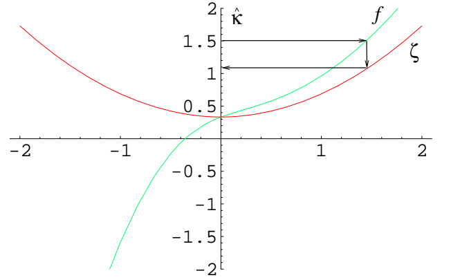
FIG. 14: The function f(x) (green/light) and \zeta_1(x) (red/dark) defined in the text. One can read off \zeta_1 as a function of \hat{\kappa} as follows: The curve y = f(x) yields \tilde{\lambda}_{\hat{\kappa}} (x axis) from \hat{\kappa} (y axis) and in turn, one reads \zeta_1(\tilde{\lambda}_{\hat{\kappa}}) (y axis) from \tilde{\lambda}_{\hat{\kappa}} (x axis) using the curve y = \zeta_1(x) . This is indicated by the arrows. The result is plotted in Fig. 15
