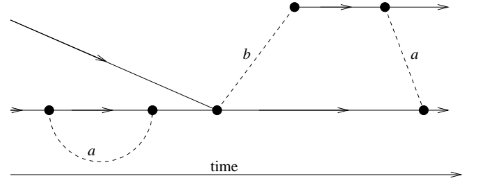
FIG. 11: Self-avoidance plus branching.
