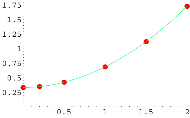
FIG. 13: \zeta_1 = \zeta/\epsilon as a function of \tilde{\lambda} for LR elasticity. Note that \zeta_1(-\tilde{\lambda}) = \zeta_1(\tilde{\lambda}) .
