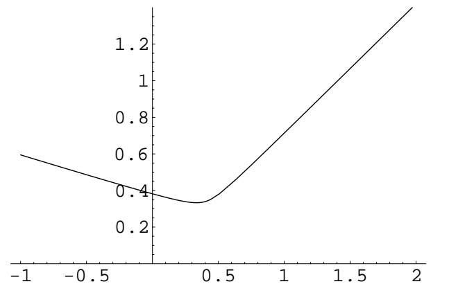
FIG. 15: \zeta_1(\hat{\kappa}) , using \zeta(\tilde{\lambda}) and \tilde{\lambda} = f^{-1}(\hat{\kappa})
