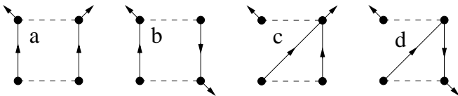
FIG. 3: 1-loop dynamical diagrams correcting \hat{\Delta}
