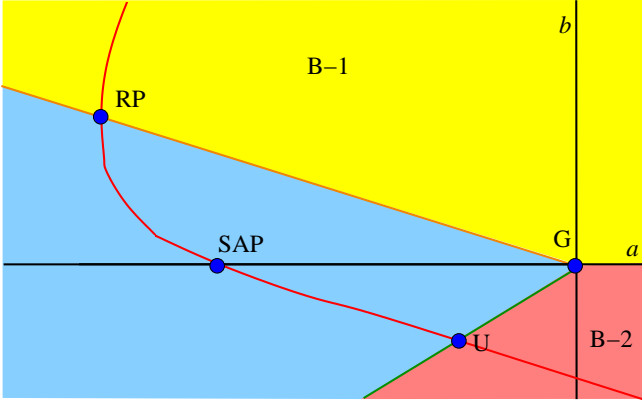
FIG. 9: The three phases of the flow-diagrams on figure 6.
