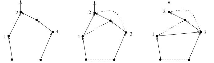
FIG. 5: Figure explaining the non-renormalization of \hat{\lambda} , see main text.
